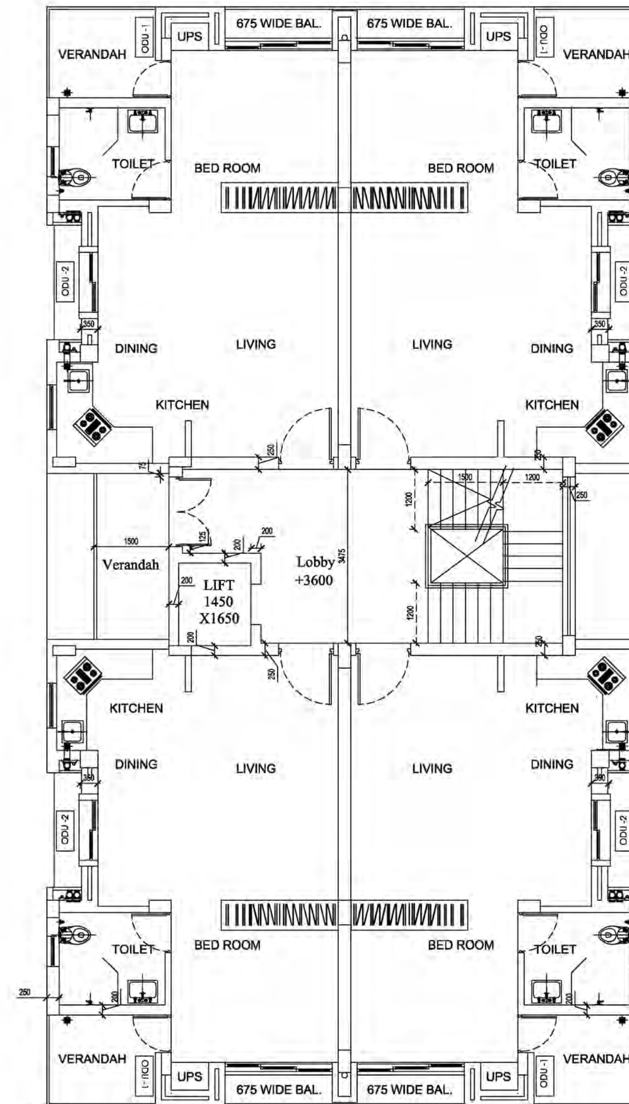
1ST FLOOR PLAN (Studio Block)
