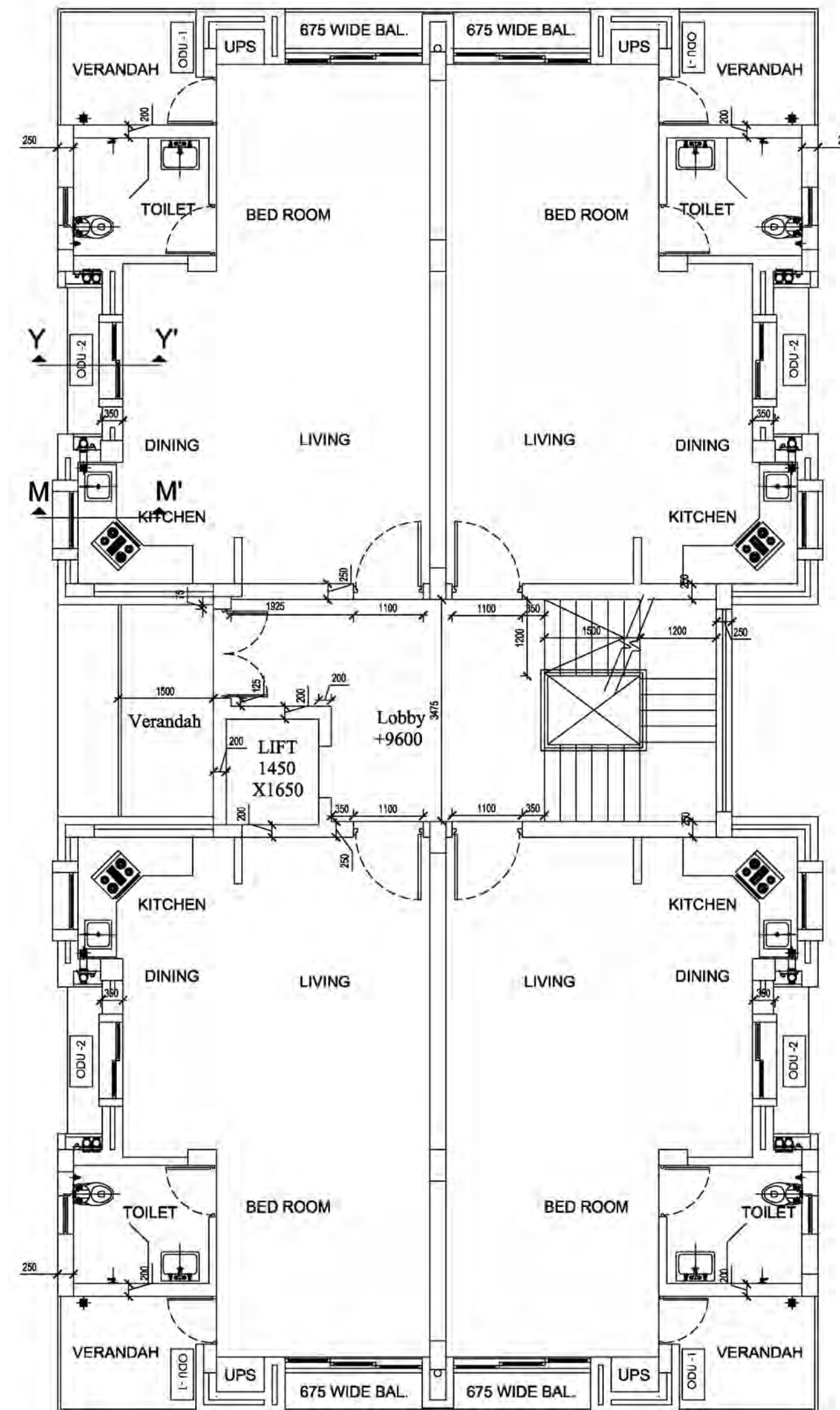
3RD FLOOR PLAN (Studio Block)
