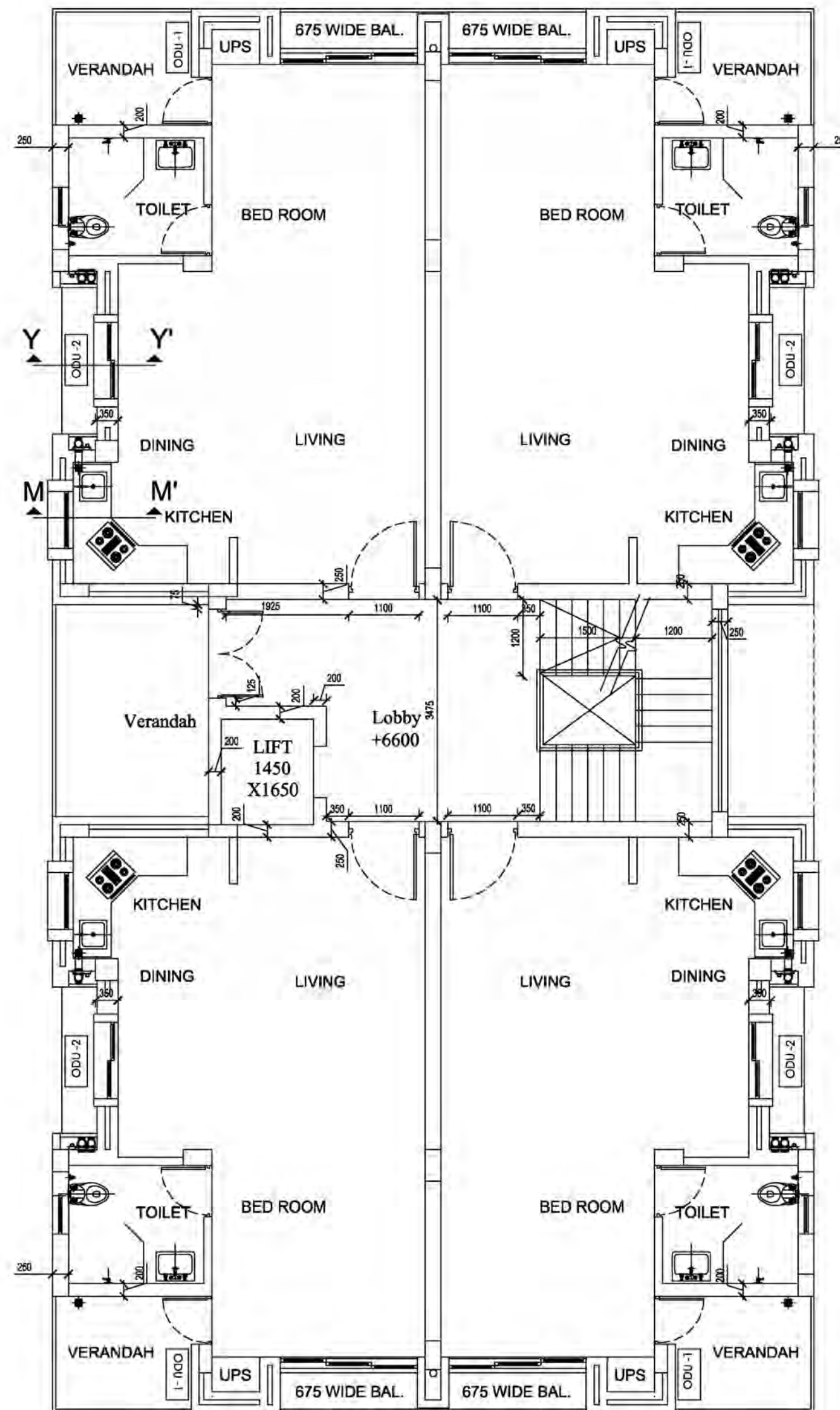
2nd FLOOR PLAN (Studio Block)
