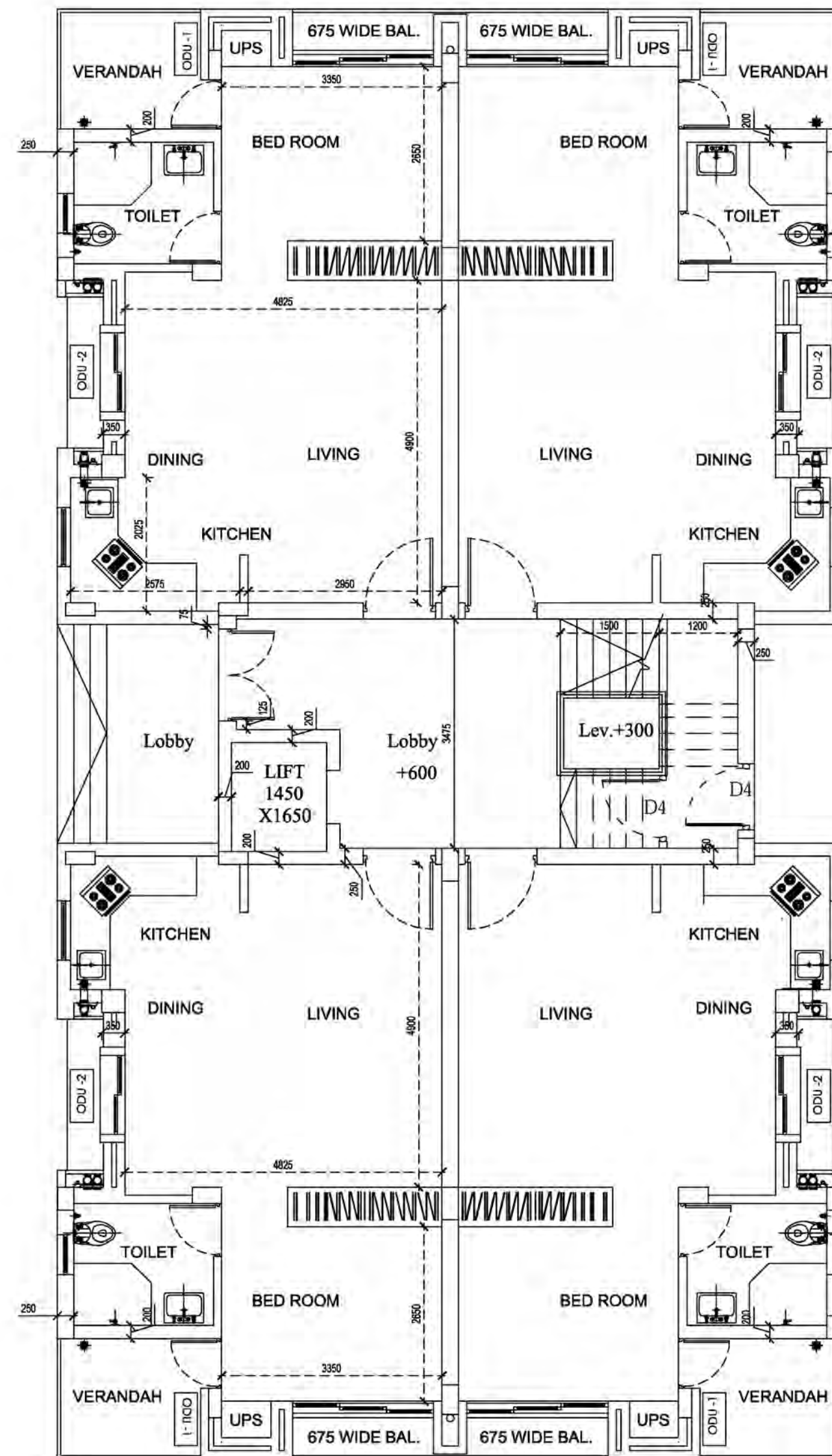
GROUND FLOOR PLAN (Studio Block)
