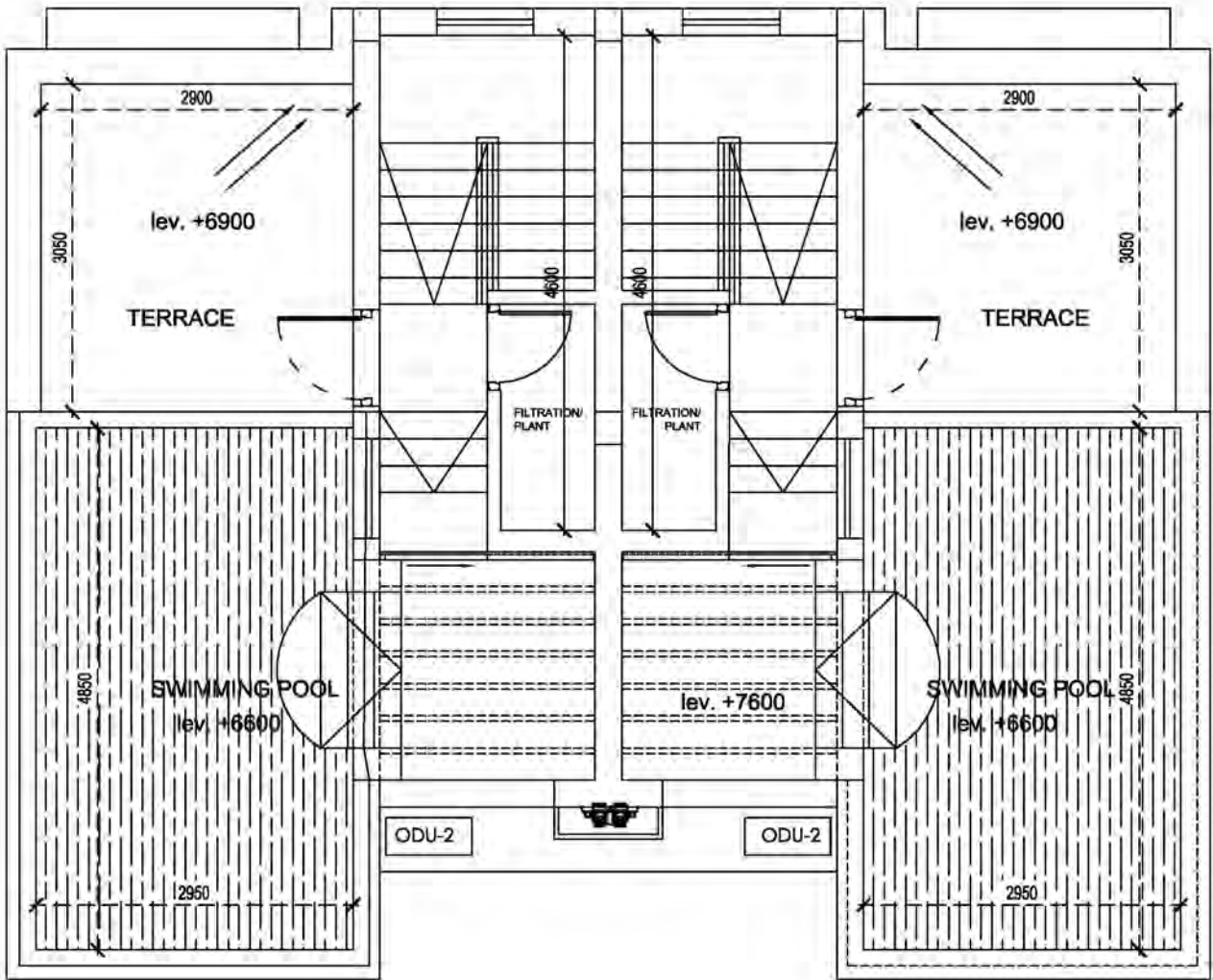
ROOF PLAN
