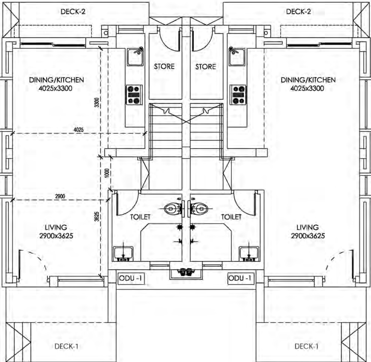
GROUND FLOOR PLAN ~ Duplex
